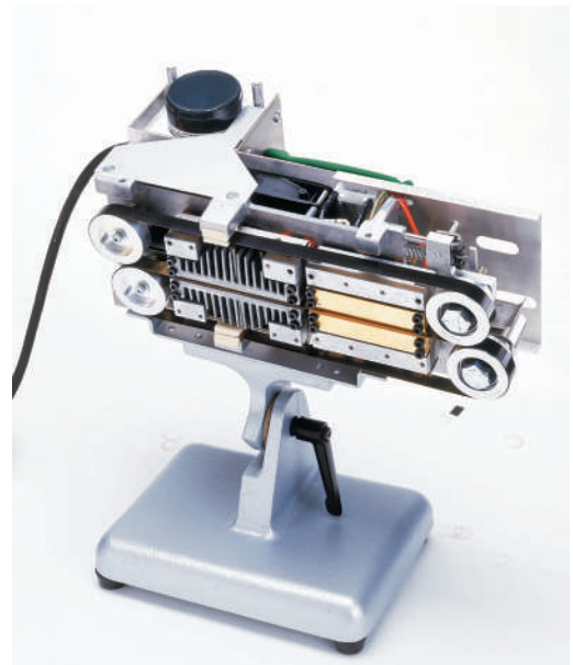
Inside mechanics of the HS-CII Hand Sealer
